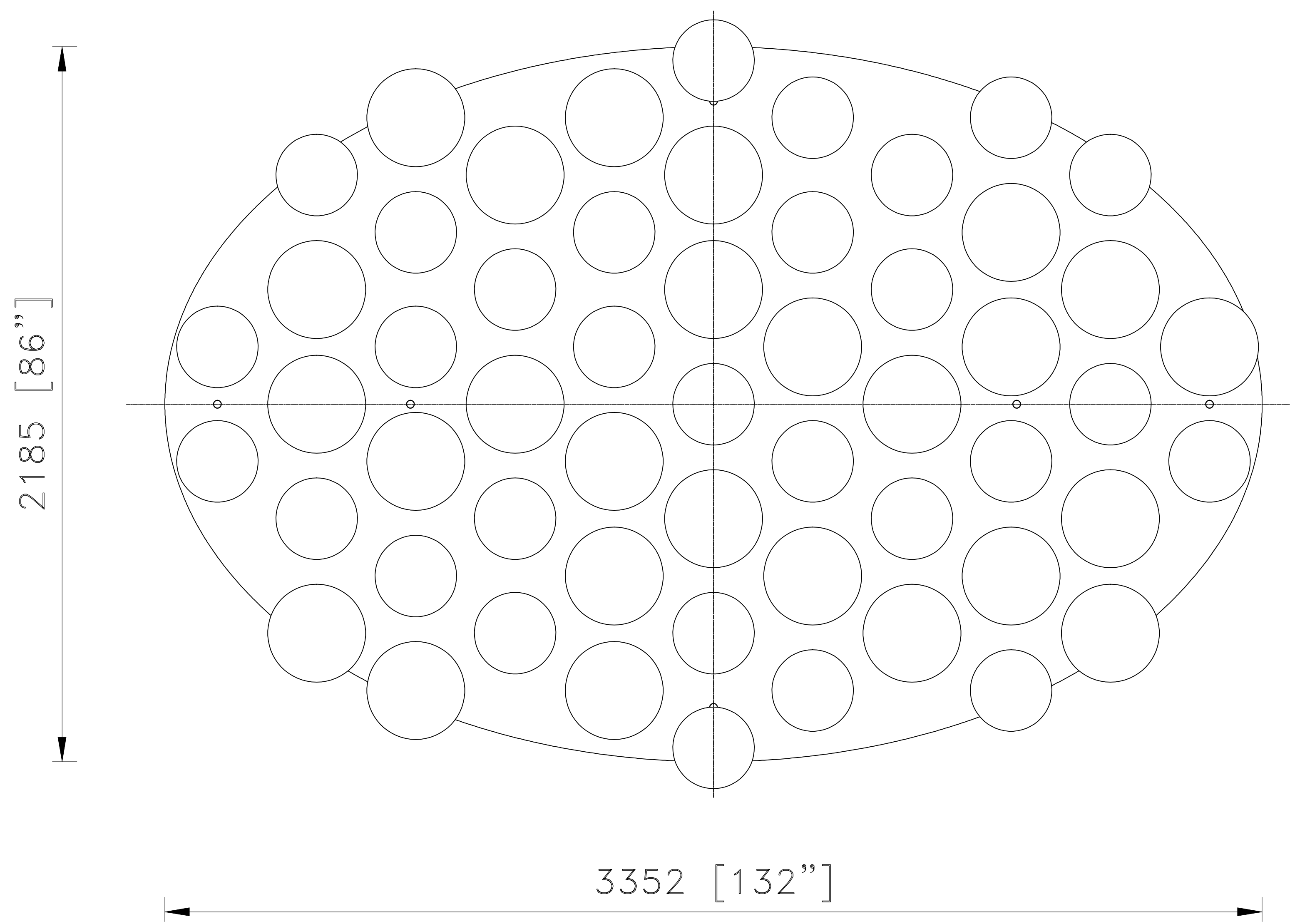
FRONT VIEW
