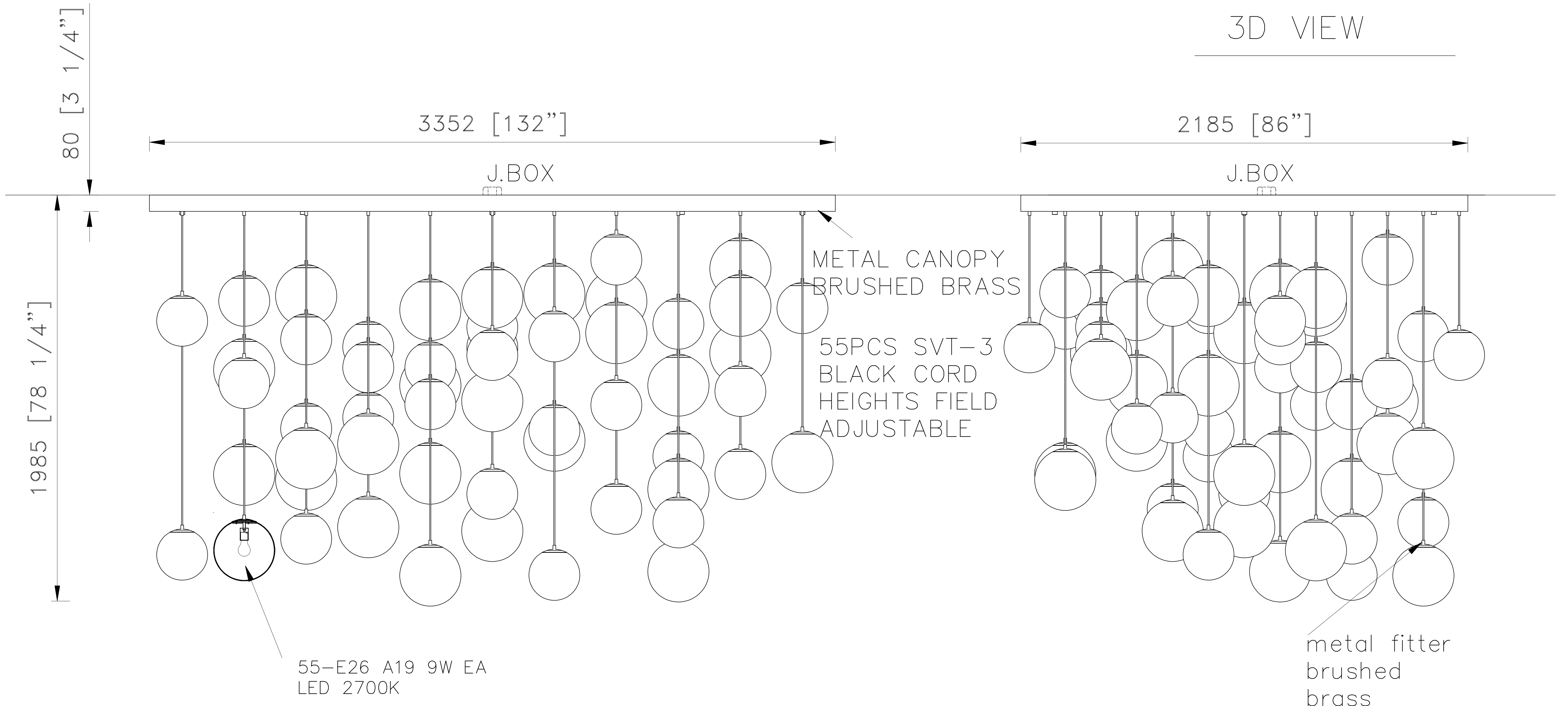
TOP VIEW
